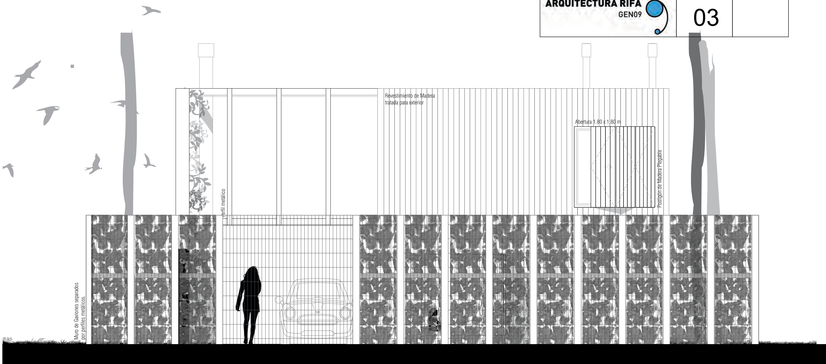
FACHADA PRINCIPAL esc 1.50
